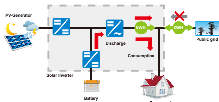
No PV energy, and the consumption from household is supplied by the battery
