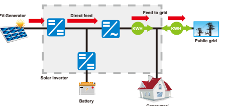
No consumption from household and the battery is fully charged
