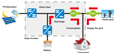
No PV energy and battery is fully discharged
